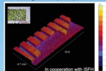
Contact wrap through via laser milling
