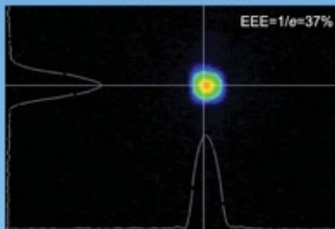
2D square top-hat beam
